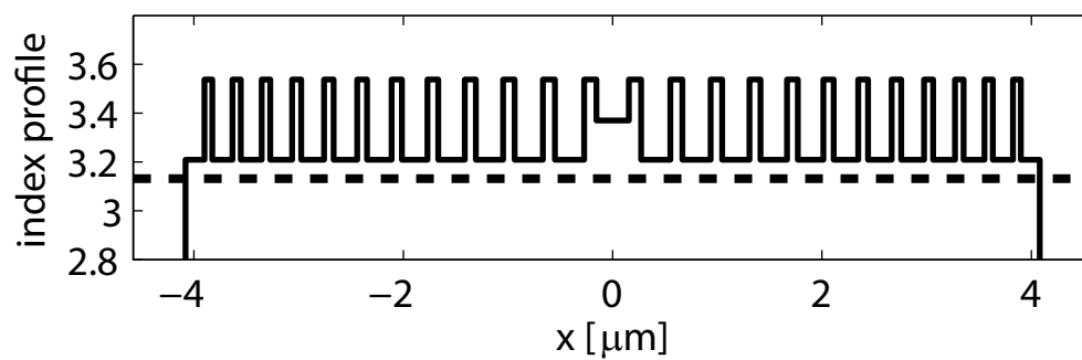
index profile of TE_0(2\omega)
