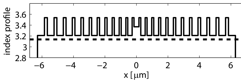
index profile of \text{TE}_0(2\omega)
